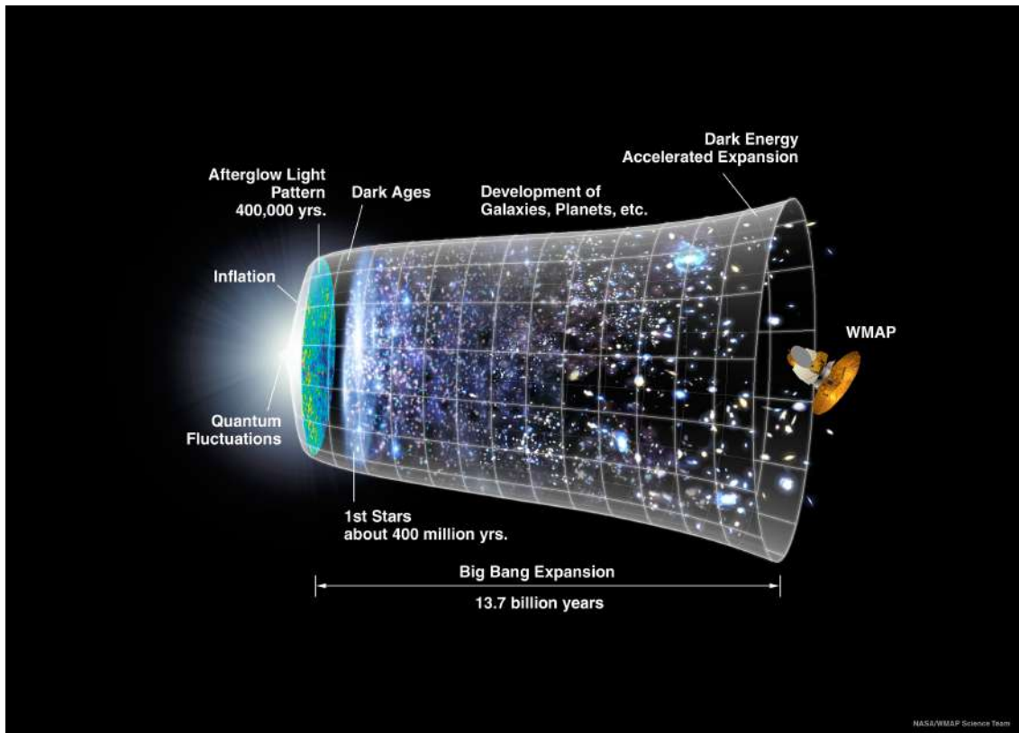
La historia del Universo (Credito: NASA/WMAP Science Team)
